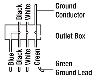
Figure 10 Diagram indicates light kit wiring.
